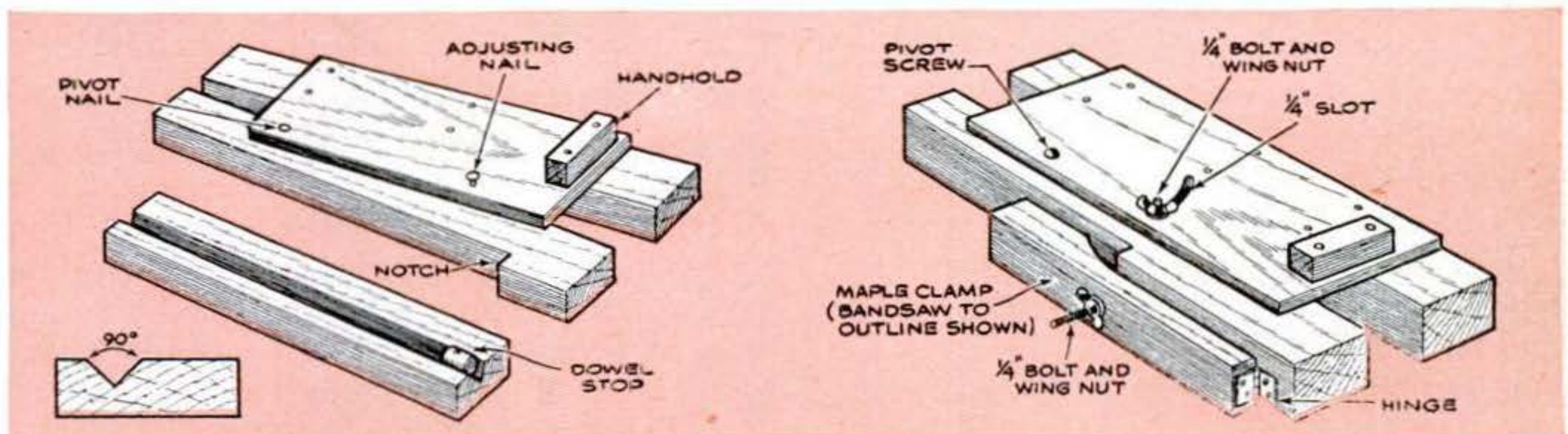
THE QUICK-SETTING JIG does a production run of model-airplane wings. Stop is clamped to fence.
